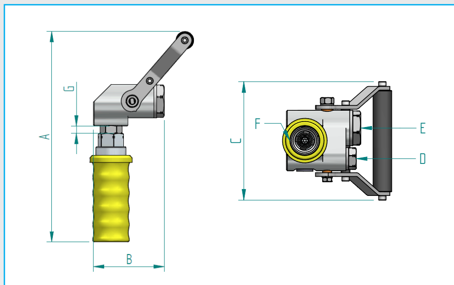
FV103-11B-9 - P36 Light Duty Transit Nozzle
